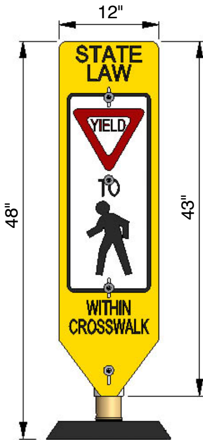
SR948PCD44XXX-D (SHOWN WITH SRPJ5WFY40 VERTICAL PANEL)
